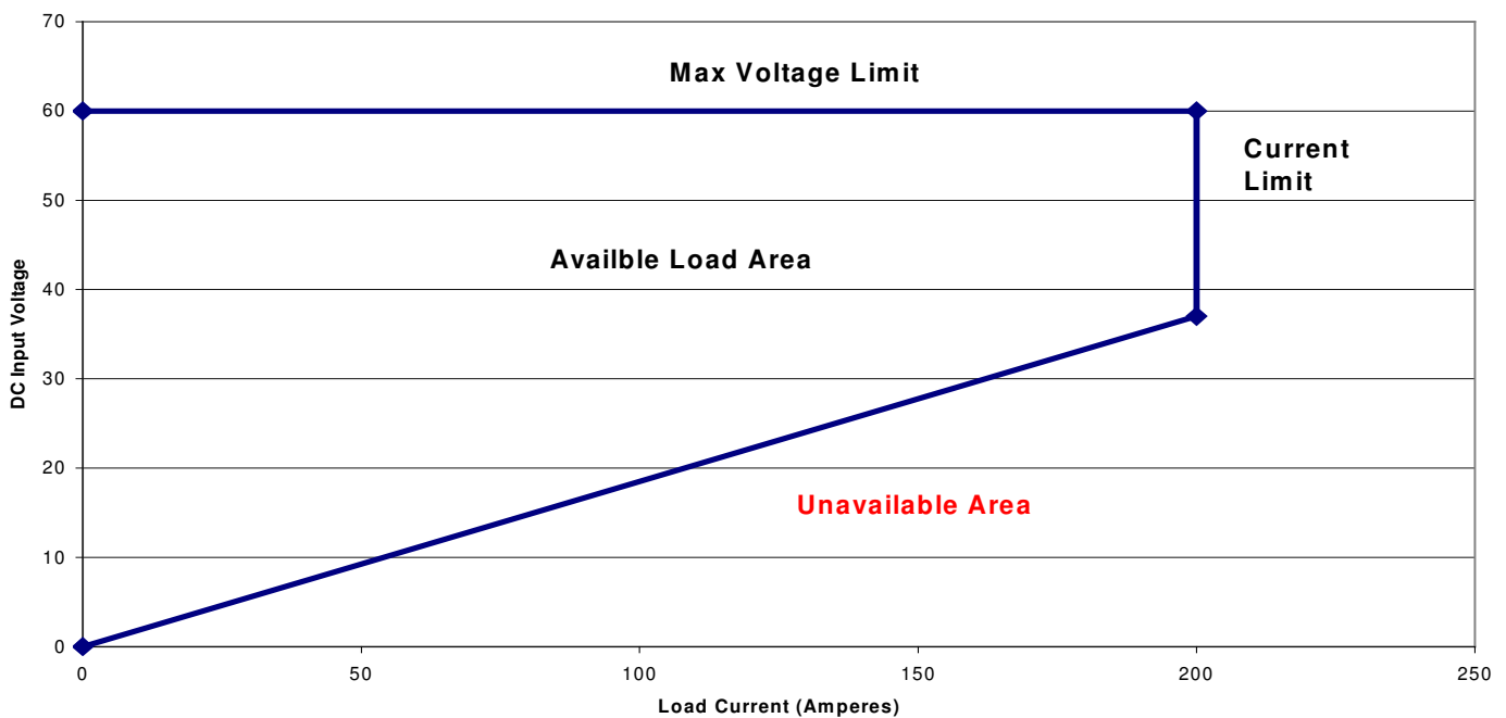
48V / 200A Model EL12-48M Operating Area
