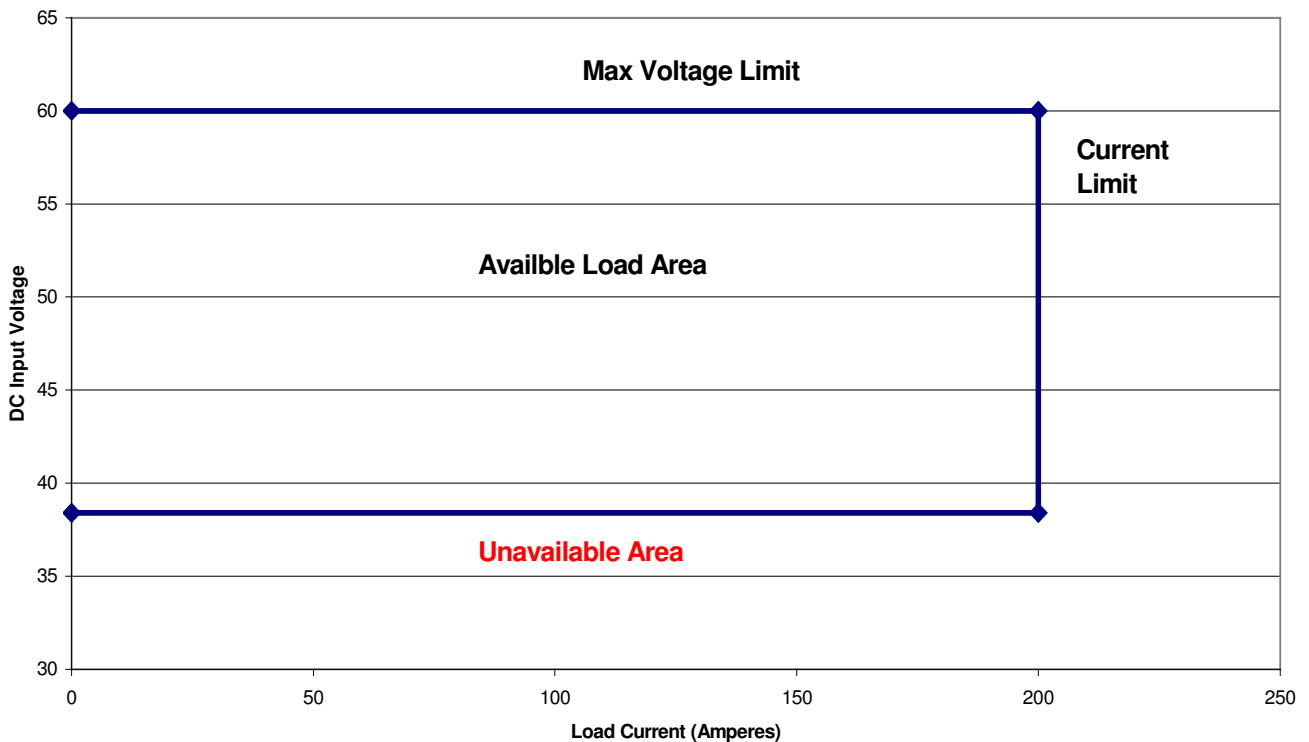
48V / 200A Model Operating Area
