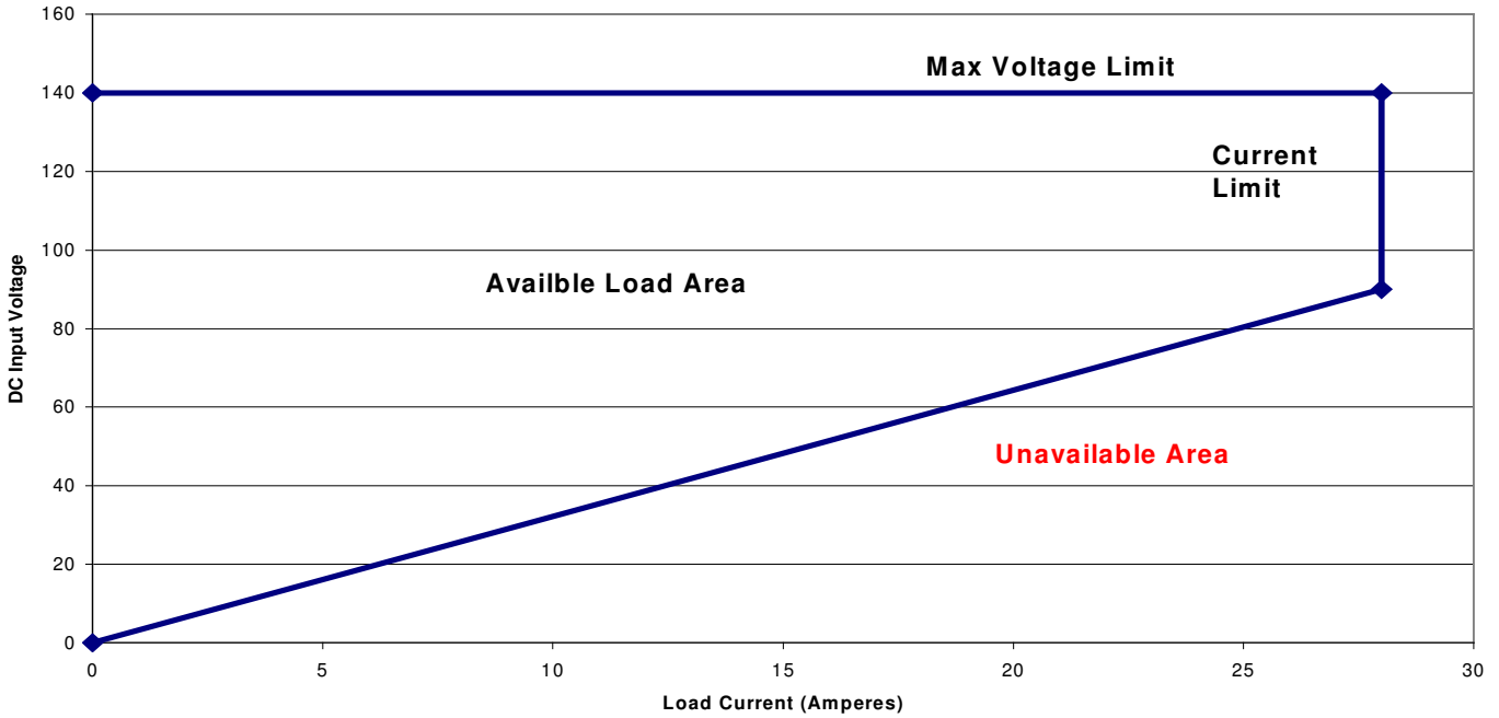
140V Range Operating Area
