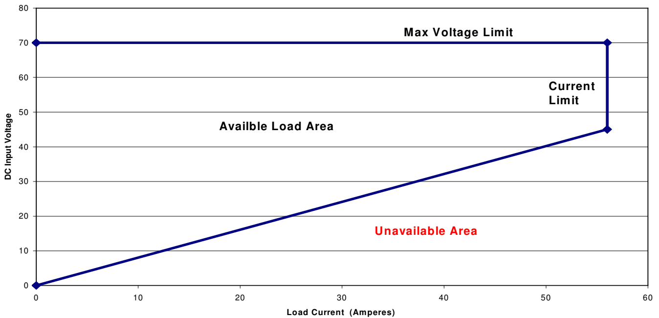
70V Range Operating Area
