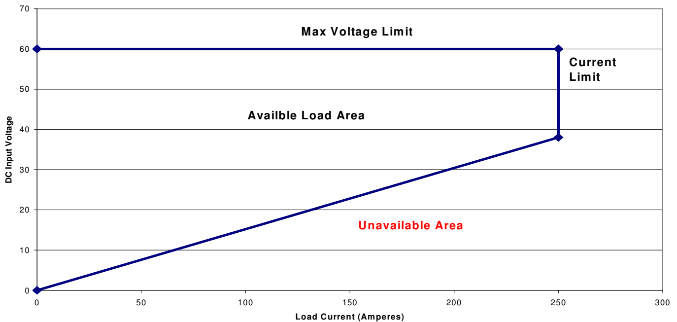
48V / 250A Model EL15-48M Operating Area
