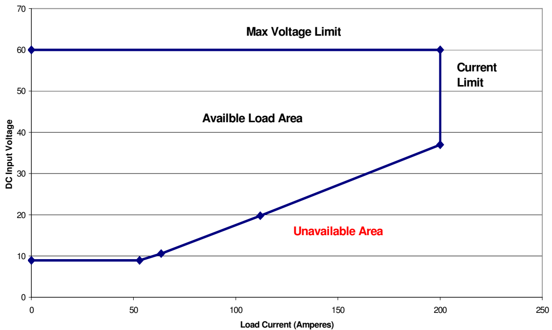
48V / 200A Model BD12-48P-24/12 Operating Area
